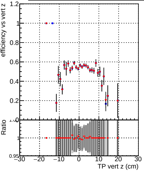
Efficiency vs TP vert z (cm) Legend: DQM_TT_ORIGINAL (blue squares) DQM_TT_MODIFIED_propToPlane_PRRVersionFINAL (red circles)
