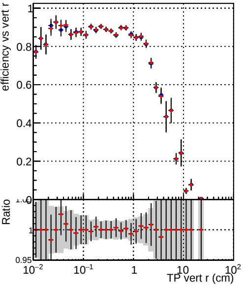
Efficiency vs TP vert r (cm) Legend: DQM_TT_ORIGINAL DQM_TT_MODIFIED_propToPlane_PRRVersionFINAL
