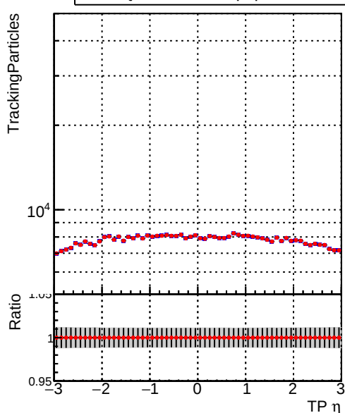
N of simulated tracks vs TP \eta Legend: DQM_TT_ORIGINAL (blue squares), DQM_TT_MODIFIED_propToPlane_PRVersionFINAL (red circles)
