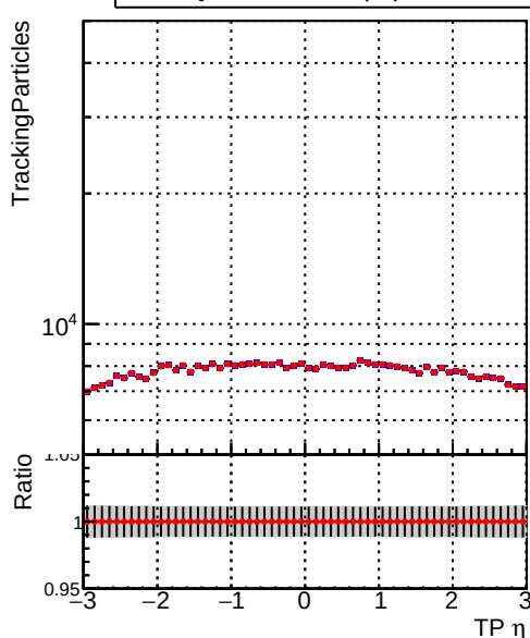
N of simulated tracks vs TP \eta Legend: DQM_TT_ORIGINAL (blue squares), DQM_TT_MODIFIED_propToPlane_PRVersionFINAL (red stars)
