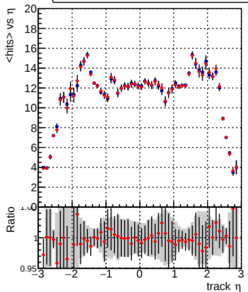
mean hits vs \eta Legend: DQM_TT_ORIGINAL (blue line), DQM_TT_MODIFIED_propToPlane_PRVersioniFINAL (red line)
