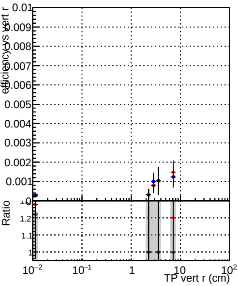
Efficiency vs vertpos DQM_TT_ORIGINAL DQM_TT_MODIFIED_layerProcv2 DQM_TT_MODIFIED_layerProcv2_OctoberVersion
