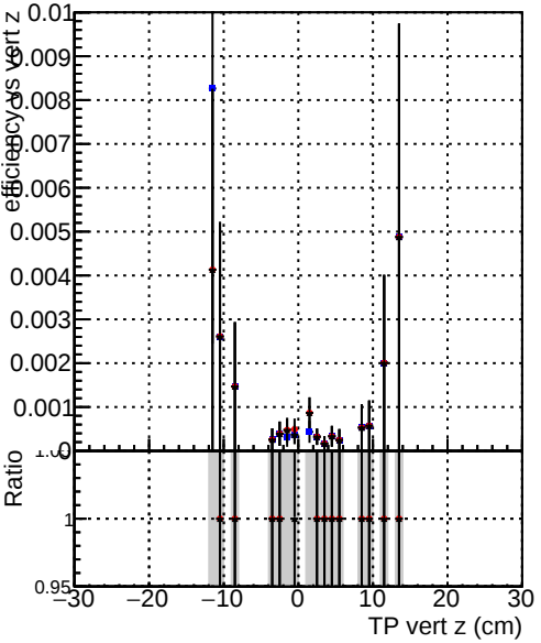
Efficiency vs vertpos DQM_TT_ORIGINAL DQM_TT_MODIFIED_layerProcv2 DQM_TT_MODIFIED_layerProcv2_OctoberVersion
