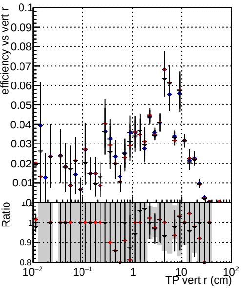
Efficiency vs TP vert r (cm) Legend: DQM_TT_ORIGINAL (blue circles) DQM_TT_MODIFIED_layerProcv2 (red circles) DQM_TT_MODIFIED_layerProcv2_OctoberVersion (black circles)
