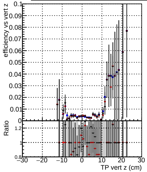
Efficiency — DQM_TT_ORIGINAL — DQM_TT_MODIFIED_layerProcv2 — DQM_TT_MODIFIED_layerProcv2_OctoberVersion
