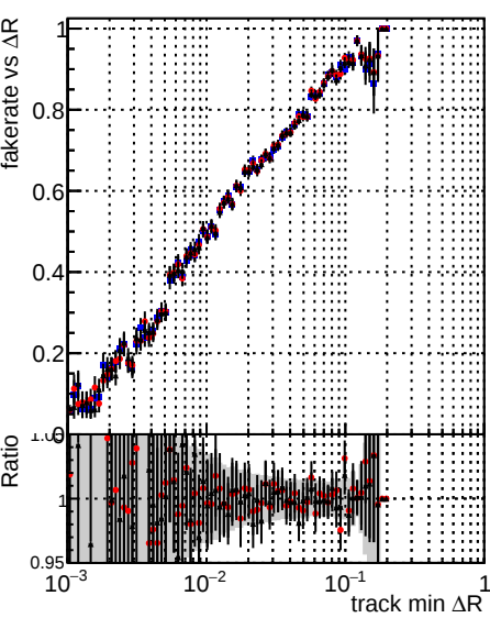
Legend: DQM TT ORIGINAL (black line with blue dots), DQM TT MODIFIED_layerProcv2 (red line with red dots), DQM TT MODIFIED_layerProcv2_OctoberVersion (black line with black dots)
