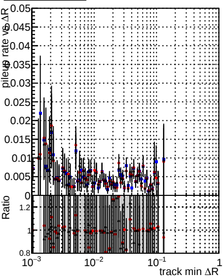
Legend: DQM TT ORIGINAL (black line with blue dots), DQM TT MODIFIED_layerProcv2 (red line with red dots), DQM TT MODIFIED_layerProcv2_OctoberVersion (black line with black dots)
