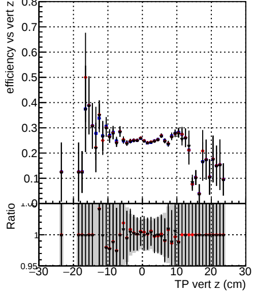
Efficiency vs. TP vert z (cm) Legend: - DQM_TT_ORIGINAL (blue line with circles) - DQM_TT_MODIFIED_layerProcv2 (red line with circles) - DQM_TT_MODIFIED_layerProcv2_OctoberVersion (black line with circles)
