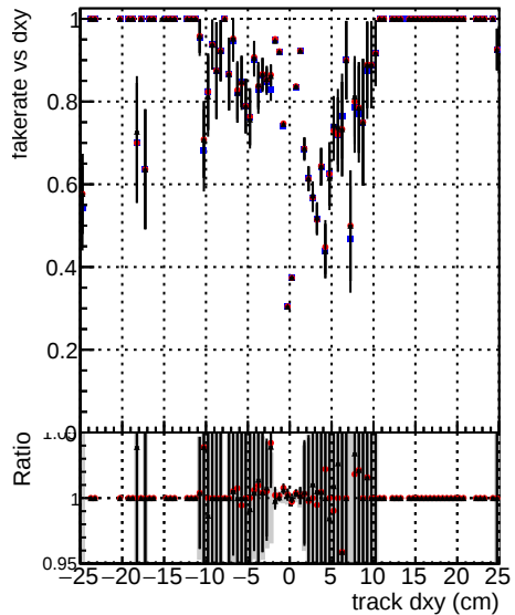
Fake rate vs d DOM TT ORIGINAL layerProcV2 DOM TT MODIFIED layerProcV2 OctoberVersion
