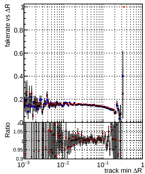
Legend for Fake rate vs \Delta R , Duplicates Rate vs \Delta R , and Pileup rate vs \Delta R : DQM TT ORIGINAL (black circles) DQM TT MODIFIED_layerProcV2 (red circles) DQM TT MODIFIED_layerProcV2_OctoberVersion (blue circles)
