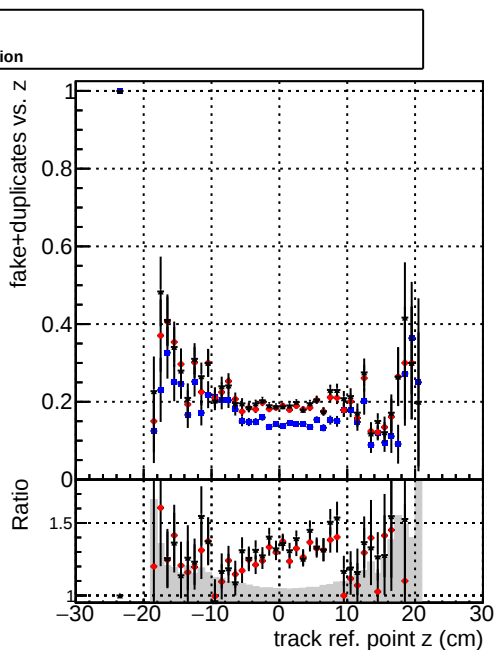
fake+duplicates vs track ref. point z
