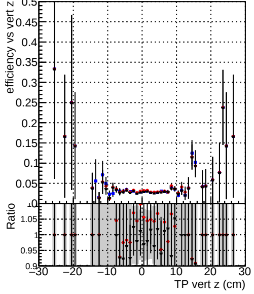
Efficiency vs. TP vert z (cm) Legend: - DQM_TT_ORIGINAL (blue circles) - DQM_TT_MODIFIED_layerProcv2 (red circles) - DQM_TT_MODIFIED_layerProcv2_OctoberVersion (black circles)
