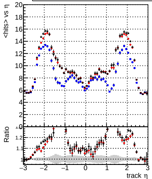
mean hit — DQM_TT_ORIGINAL — DQM_TT_MODIFIED_layerProcV2 — DQM_TT_MODIFIED_layerProcV2_OctoberVersion
