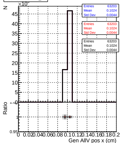
Legend: DQM_TT_ORIGINAL (blue line), DQM_TT_MODIFIED_layerProcV2 (red line), DQM_TT_MODIFIED_layerProcV2_OctoberVersion (black line)
