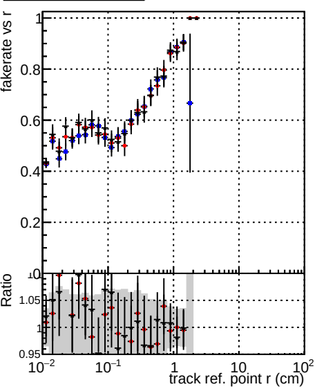
—●— DOM TT ORIGINAL —●— DOM TT MODIFIED —●— DOM TT MODIFIED layerProcv2
