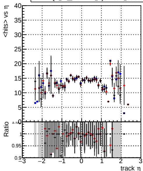
mean hit — DQM_TT_ORIGINAL — DQM_TT_MODIFIED_layerProcv2 — DQM_TT_MODIFIED_layerProcv2_OctoberVersion
