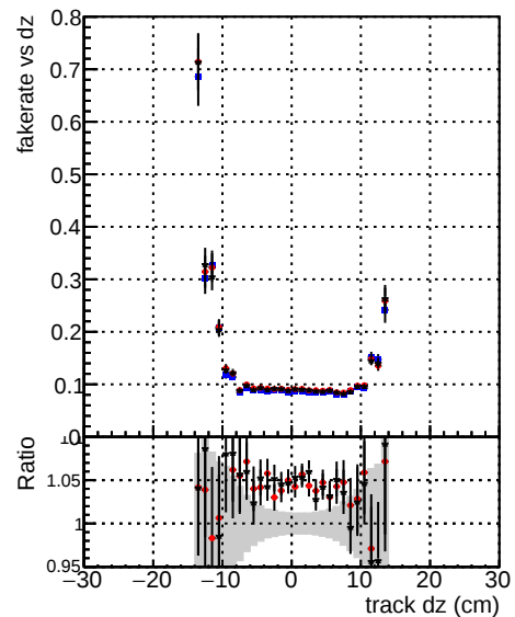
Fake rate vs dz —•— DOM TT ORIGINAL —•— DOM TT MODIFIED —•— layerProcv2 —•— layerProcv2 OctoberVersion
