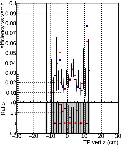
Efficiency vs vertpos Legend: DQM_TT_ORIGINAL DQM_TT_MODIFIED_layerProcv2 DQM_TT_MODIFIED_layerProcv2_OctoberVersion
