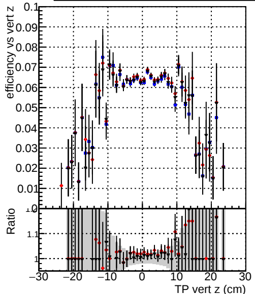
Efficiency vs vert z —●— DQM_TT_ORIGINAL —●— DQM_TT_MODIFIED_layerProcv2 —●— DQM_TT_MODIFIED_layerProcv2_OctoberVersion
