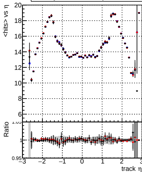
mean hits vs \eta — DQM_TT_ORIGINAL — DQM_TT_MODIFIED_layerProcV2 — DQM_TT_MODIFIED_layerProcV2_OctoberVersion
