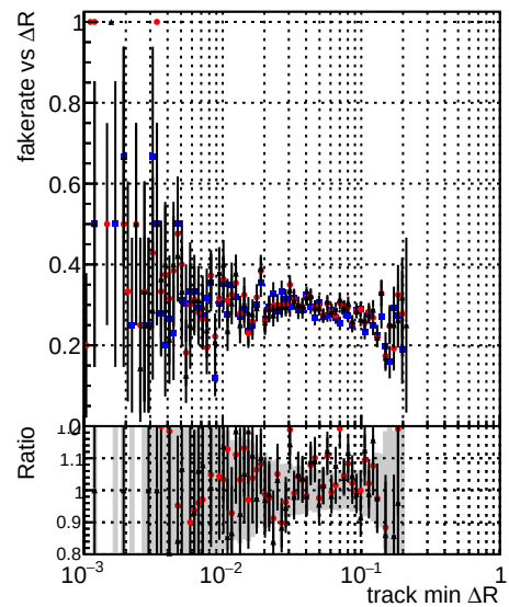
Legend: DQM TT ORIGINAL (black), DQM TT MODIFIED (red), DQM TT MODIFIED layerProcv2 (blue). Fake rate vs \Delta R(\text{track, jet})
