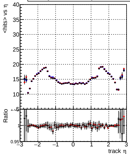
mean hits vs \eta — DQM_TT_ORIGINAL — DQM_TT_MODIFIED_layerProcV2 — DQM_TT_MODIFIED_layerProcV2_OctoberVersion
