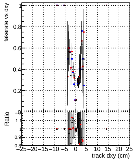
Fake rate vs d DOM TT ORIGINAL layerProcv2 OctoberVersion DOM TT MODIFIED layerProcv2 OctoberVersion
