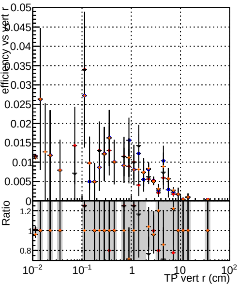
Efficiency vs vertpos Series Color Shape Line Style DQM TT ORIGINAL Blue Circle Solid DQM TT MODIFIED layerProcv2 Red Circle Solid DQM TT MODIFIED layerProcv2_windows Black Circle Solid DQM TT MODIFIED layerProcv2_windows_hits Orange Circle Solid
