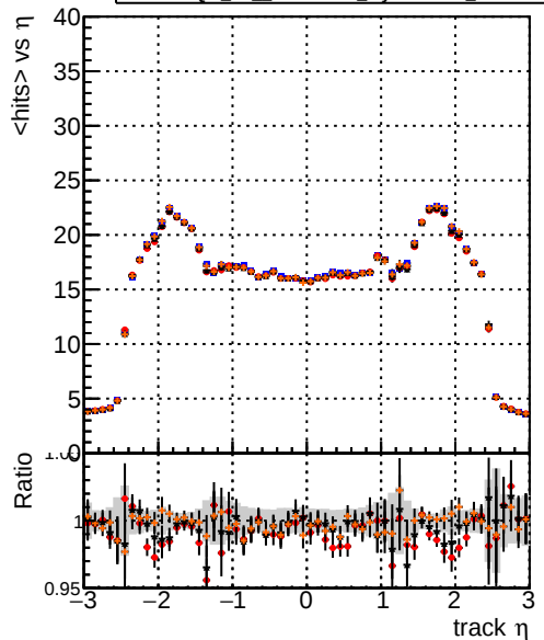
mean hits vs \eta DQM_TT ORIGINAL layerProc2 DQM_TT MODIFIED layerProc2_windows DQM_TT MODIFIED layerProc2_windows_hits
