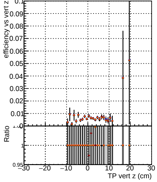
Efficiency vs. TP vert z (cm) Series Color Shape Line Style DQM TT ORIGINAL Blue Circle Solid DQM TT MODIFIED layerProcv2 Red Circle Solid DQM TT MODIFIED layerProcv2_windows Black Circle Solid DQM TT MODIFIED layerProcv2_windows_hits Orange Circle Dashed
