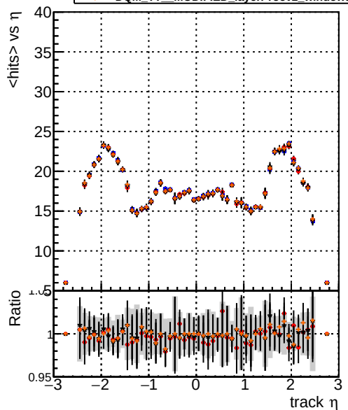
mean hits vs \eta Legend: DQM_TT ORIGINAL layerProcv2 (blue line with circles), DQM_TT MODIFIED layerProcv2 (red line with circles), DQM_TT MODIFIED layerProcv2_windows (black line with circles), DQM_TT MODIFIED layerProcv2_windows_hits (orange line with circles)
