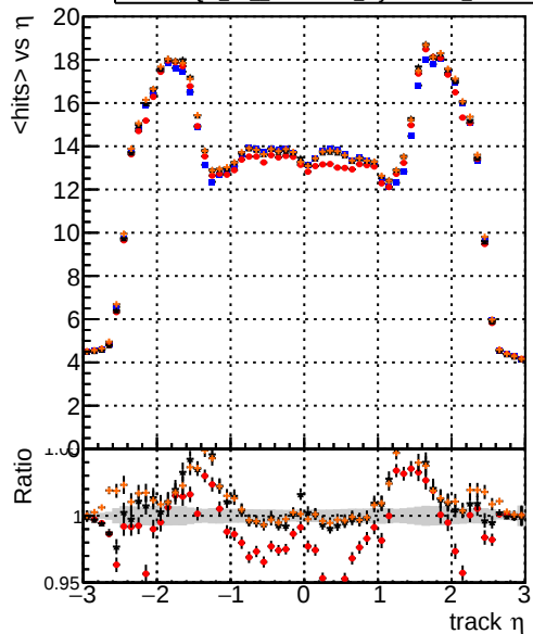
mean hits vs \eta Legend: DQM_TT ORIGINAL (blue line), DQM_TT MODIFIED layerProc2 (red line), DQM_TT MODIFIED layerProc2_windows (black line), DQM_TT MODIFIED layerProc2_windows_hits (orange line)
