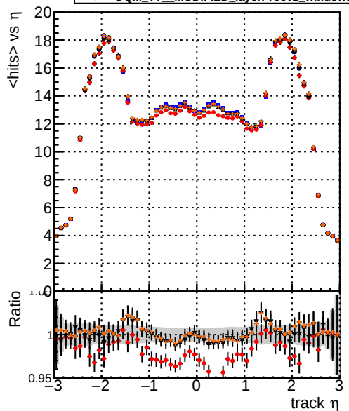
mean hits DQM_TT_ORIGINAL DQM_TT_MODIFIED_layerProc2 DQM_TT_MODIFIED_layerProc2_windows DQM_TT_MODIFIED_layerProc2_windows_hits
