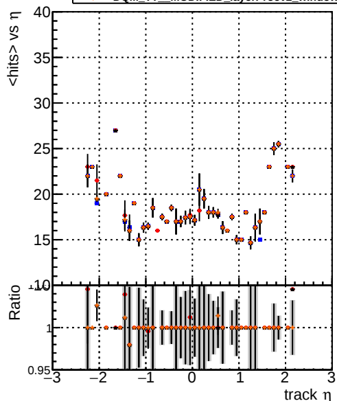
mean hits vs \eta Legend: - DQM_TT ORIGINAL layerProc2 (blue line with circles) - DQM_TT MODIFIED layerProc2 (red line with circles) - DQM_TT MODIFIED layerProc2_windows (black line with circles) - DQM_TT MODIFIED layerProc2_windows_hits (orange line with circles)
