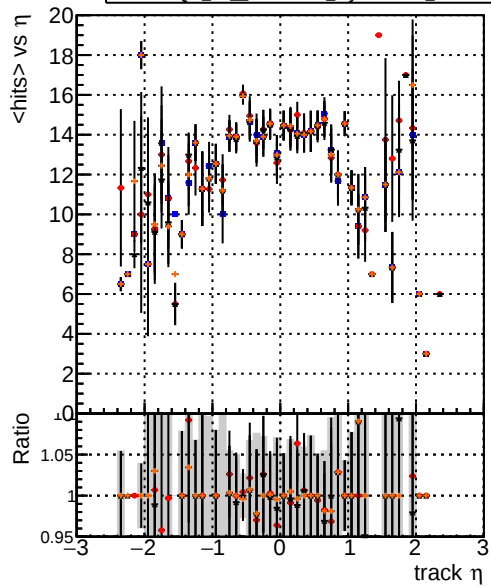
mean hits vs \eta Legend: DQM_TT ORIGINAL layerProc2 (blue), DQM_TT MODIFIED layerProc2 (red), DQM_TT MODIFIED layerProc2_windows (black), DQM_TT MODIFIED layerProc2_windows_hits (orange)
