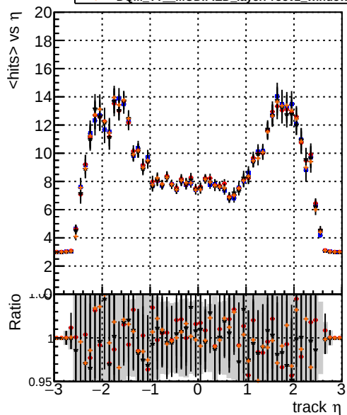
mean hits vs \eta Legend: DQM_TT ORIGINAL layerProcv2 (blue line), DQM_TT MODIFIED layerProcv2 (red line), DQM_TT MODIFIED layerProcv2_windows (grey line), DQM_TT MODIFIED layerProcv2_windows_hits (orange line)
