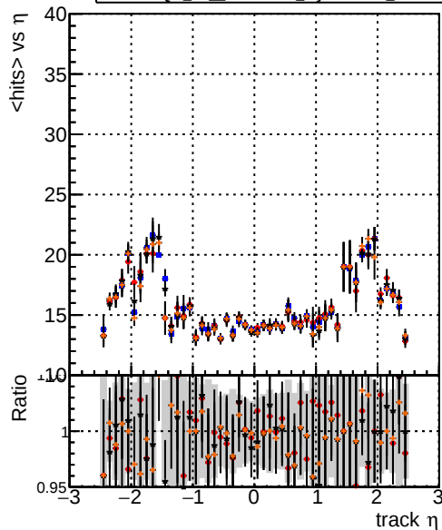
mean hits vs \eta Legend: DQM_TT_ORIGINAL DQM_TT_MODIFIED_layerProc2 DQM_TT_MODIFIED_layerProc2_windows DQM_TT_MODIFIED_layerProc2_windows_hits
