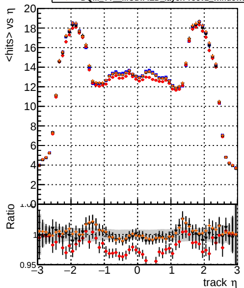
mean hits vs \eta DQM_TT ORIGINAL DQM_TT MODIFIED layerProc2 DQM_TT MODIFIED layerProc2_windows DQM_TT MODIFIED layerProc2_windows_hits
