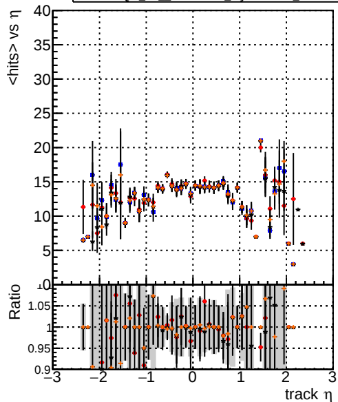
mean hits vs \eta Legend: - DQM_TT ORIGINAL layerProcv2 - DQM_TT MODIFIED layerProcv2_windows - DQM_TT MODIFIED layerProcv2_windows_hits
