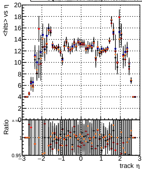
mean hits vs \eta DQM_TT ORIGINAL DQM_TT MODIFIED layerProc2 DQM_TT MODIFIED layerProc2_windows DQM_TT MODIFIED layerProc2_windows_hits
