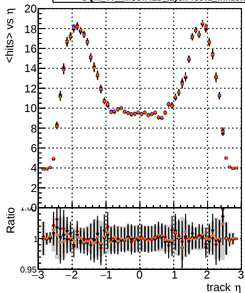
mean hits vs \eta Legend: - DQM_TT ORIGINAL layerProc2 - DQM_TT MODIFIED layerProc2 - DQM_TT MODIFIED layerProc2_windows - DQM_TT MODIFIED layerProc2_windows_hits
