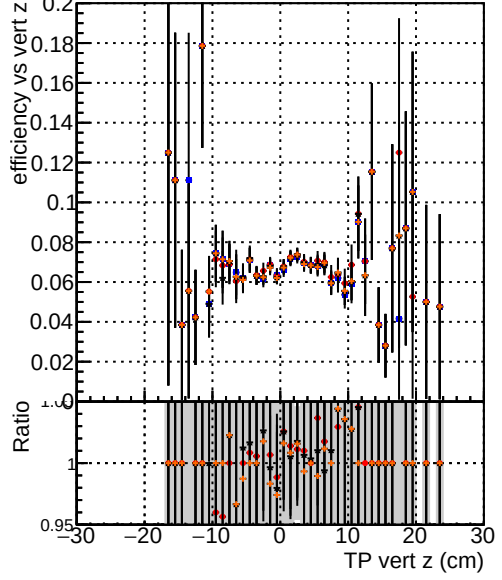
Efficiency vs vert z —●— DOM TT ORIGINAL —●— DOM TT MODIFIED layerProcv2 —●— DOM TT MODIFIED layerProcv2_windows —●— DOM TT MODIFIED layerProcv2_windows_hits
