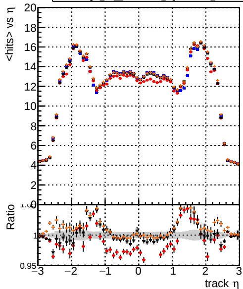
mean hits DOM TT ORIGINAL DOM TT MODIFIED layerProcv2 DOM TT MODIFIED layerProcv2_windows DOM TT MODIFIED layerProcv2_windows_hits
