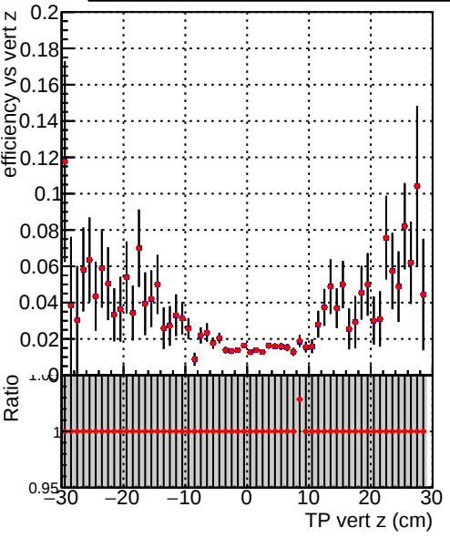
Efficiency vs TP vert z (cm) Legend: DQM_TT_ORIGINAL (Blue line with markers) DQM_TT_MODIFIED_layerProcv2_PVersion (Red line with markers)
