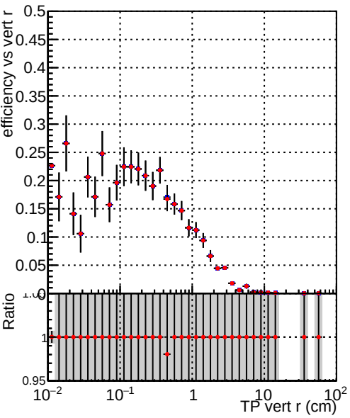
Efficiency vs TP vert r (cm) Legend: DQM_TT_ORIGINAL (blue line with dots) DQM_TT_MODIFIED_layerProcv2_PVersion (red line with dots)
