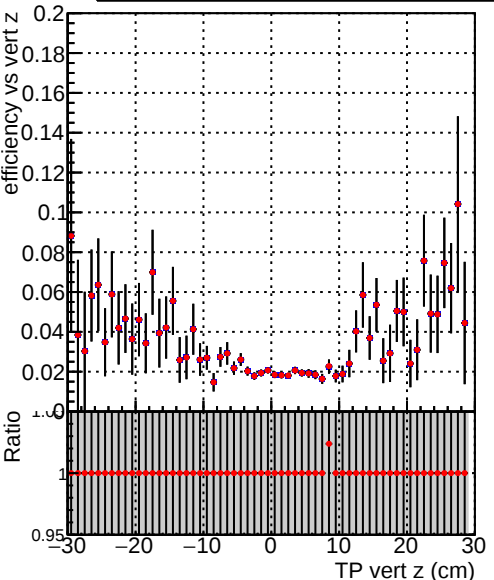
Efficiency vs TP vert z (cm) Legend: DQM_TT_ORIGINAL DQM_TT_MODIFIED_layerProcv2_PVersion
