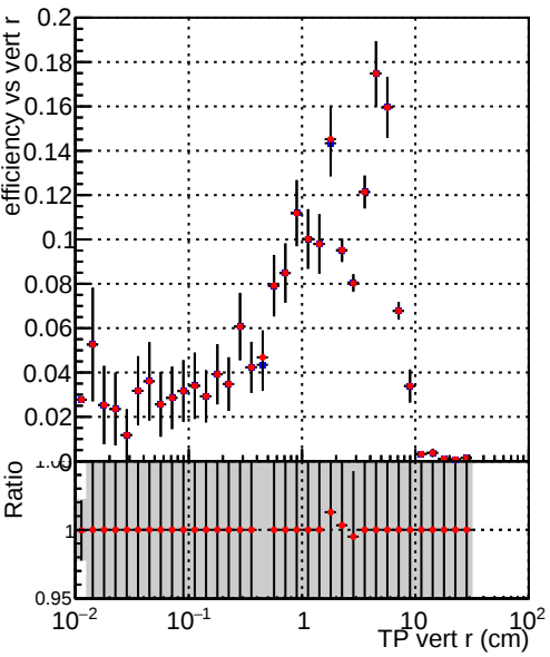
Efficiency vs TP vert r (cm) Legend: DQM_TT_ORIGINAL DQM_TT_MODIFIED_layerProcv2_PRVersion
