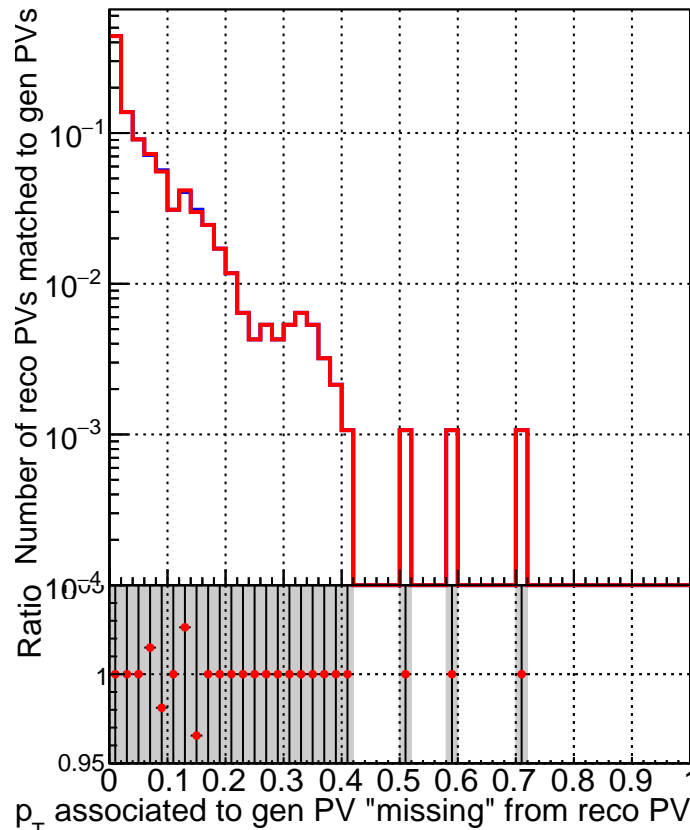
RecoPVAssoc2GenPVMatched_missing
