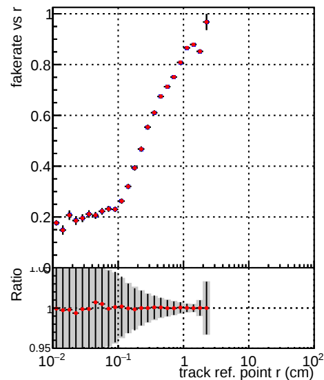
—●— DQM_TT_ORIGINAL —●— DQM_TT_MODIFIED_layerProcV2_PRVersion
