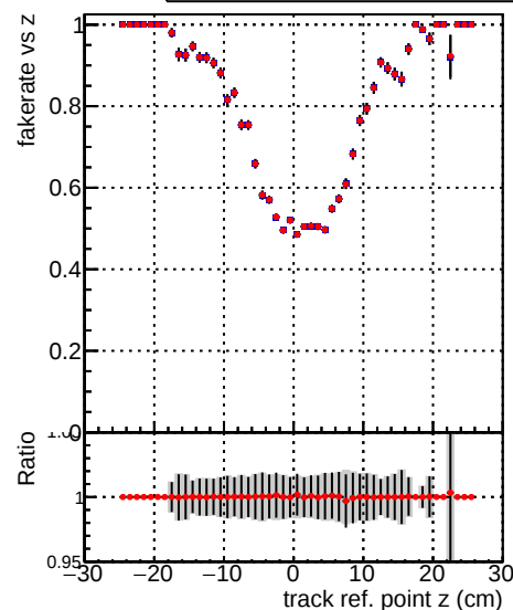
—●— DQM_TT_ORIGINAL —●— DQM_TT_MODIFIED_layerProcV2_PRVersion
