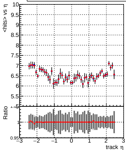
mean hits vs \eta Legend: DQM_TT_ORIGINAL (blue line with error bars), DQM_TT_MODIFIED_layerProcV2_PRVersion (red line with error bars)
