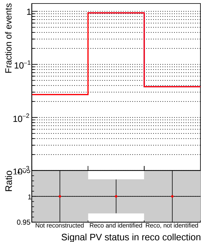
—■ DQM_TT_ORIGINAL —● DQM_TT_MODIFIED_layerProcv2_PRVersion
