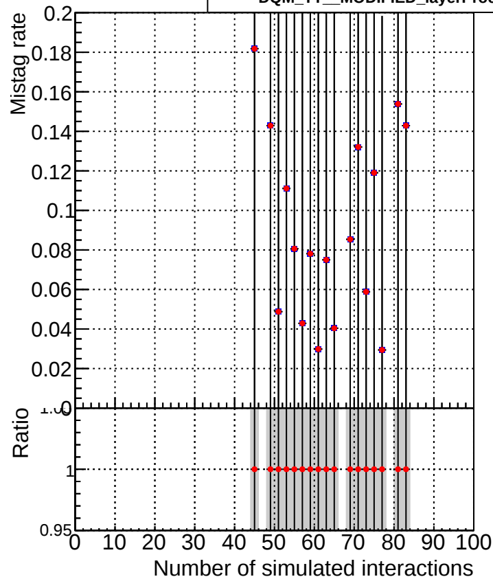
—■ DQM_TT_ORIGINAL —● DQM_TT_MODIFIED_layerProcv2_PRVersion
