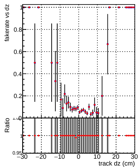
Fake rate vs dz Legend: - DQM TT ORIGINAL (blue dots) - DQM TT MODIFIED layerProcV2_PRVersion (red dots)
